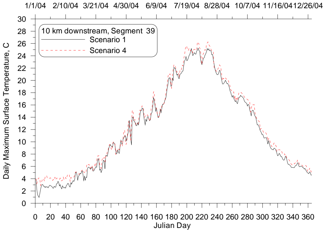
Figure 51: Daily maximum surface temperature time series at 10 km downstream from Lake Pend Oreille for the Unimpounded (4) and Existing Conditions (1) Scenarios, 2004.
