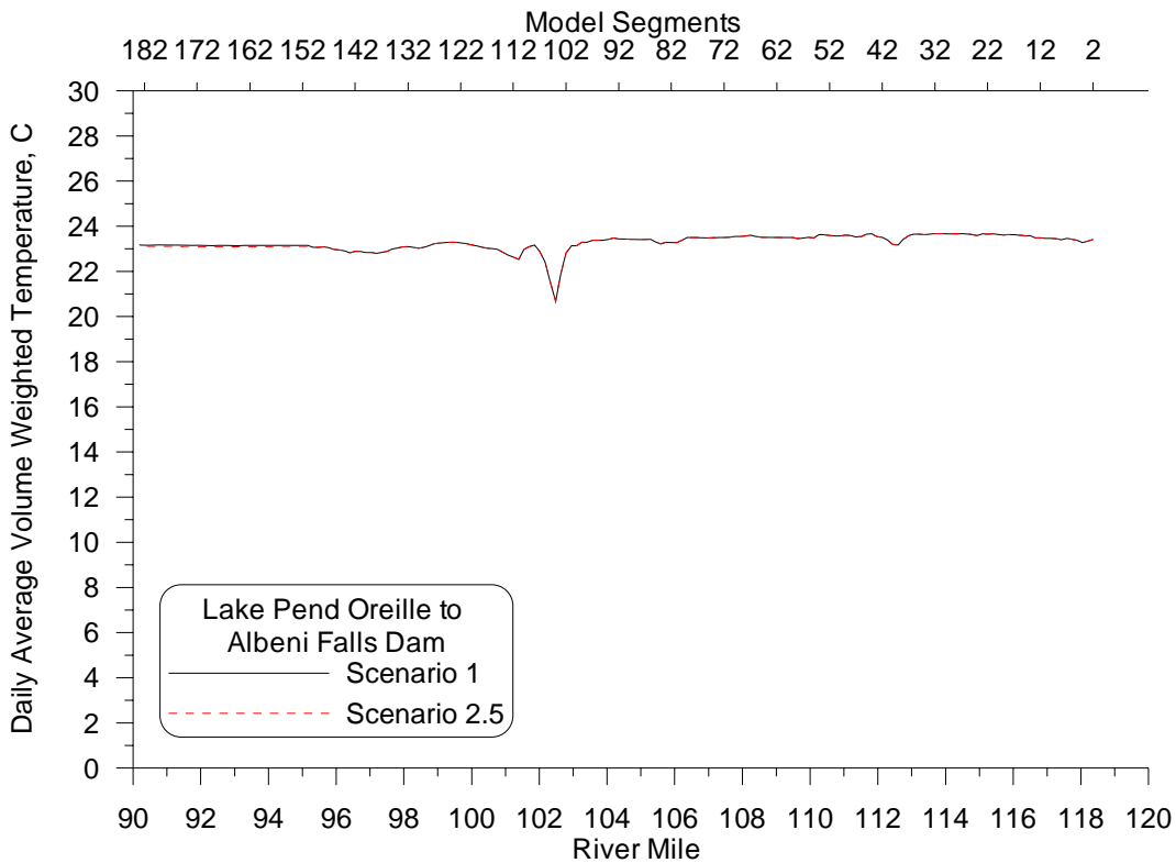
Figure 43: Daily average volume weighted temperature longitudinal profile on August 16 th , 2004 for the Impounded with no NPS (2.5) and Existing Conditions (1) Scenarios.
