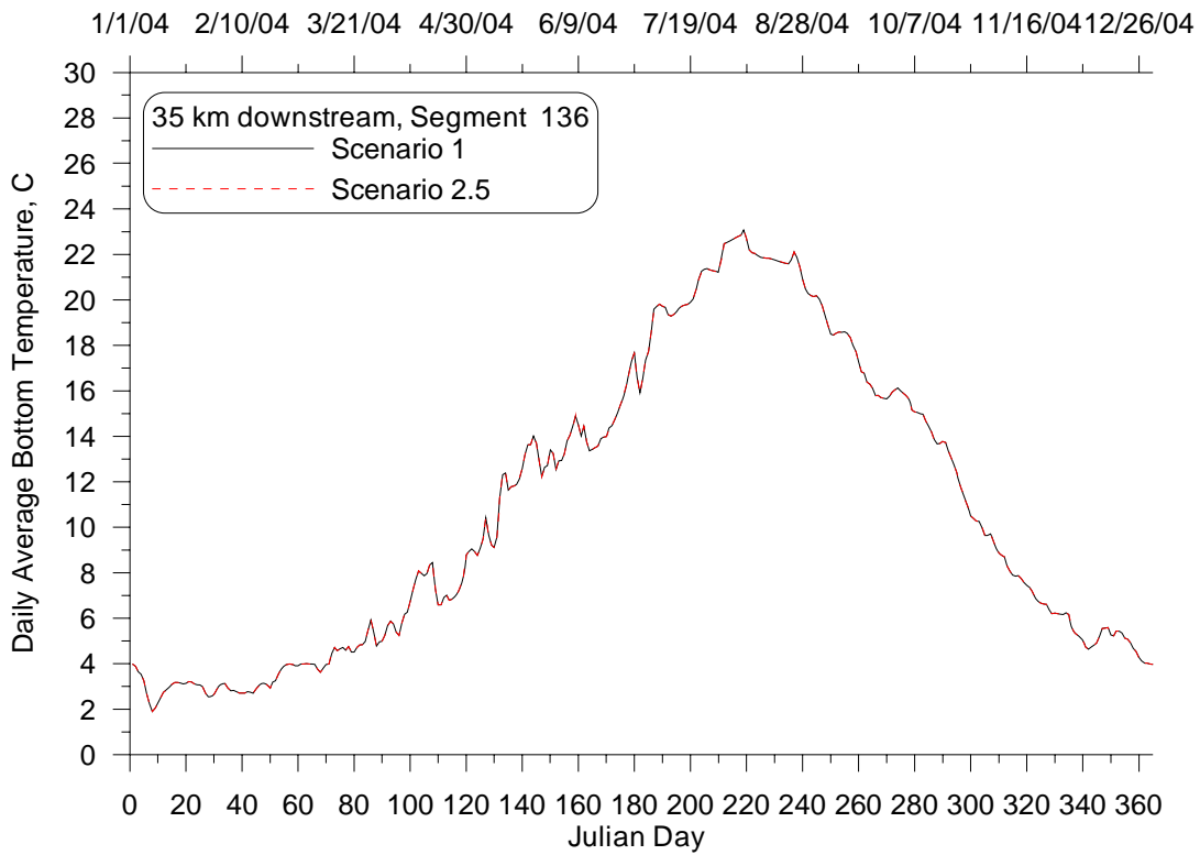
Figure 37: Daily average bottom temperature time series at 35 km downstream from Lake Pend Oreille for the Impounded with no NPS (2.5) and Existing Conditions (1) Scenarios, 2004.
