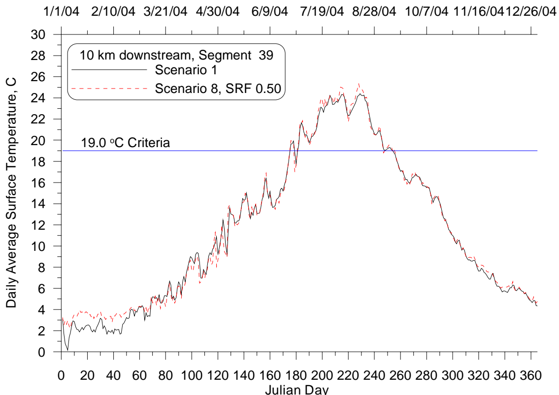
Figure 2: Daily average surface temperature time series at 10 km downstream from Lake Pend Oreille for the Natural Conditions (8) and Existing Conditions (1) Scenarios, 2004.
