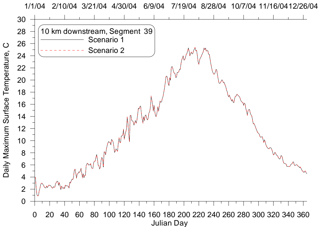
Figure 29: Daily maximum surface temperature time series at 10 km downstream from Lake Pend Oreille for the Impounded with no NPDES (2) and Existing Conditions (1) Scenarios, 2004.
