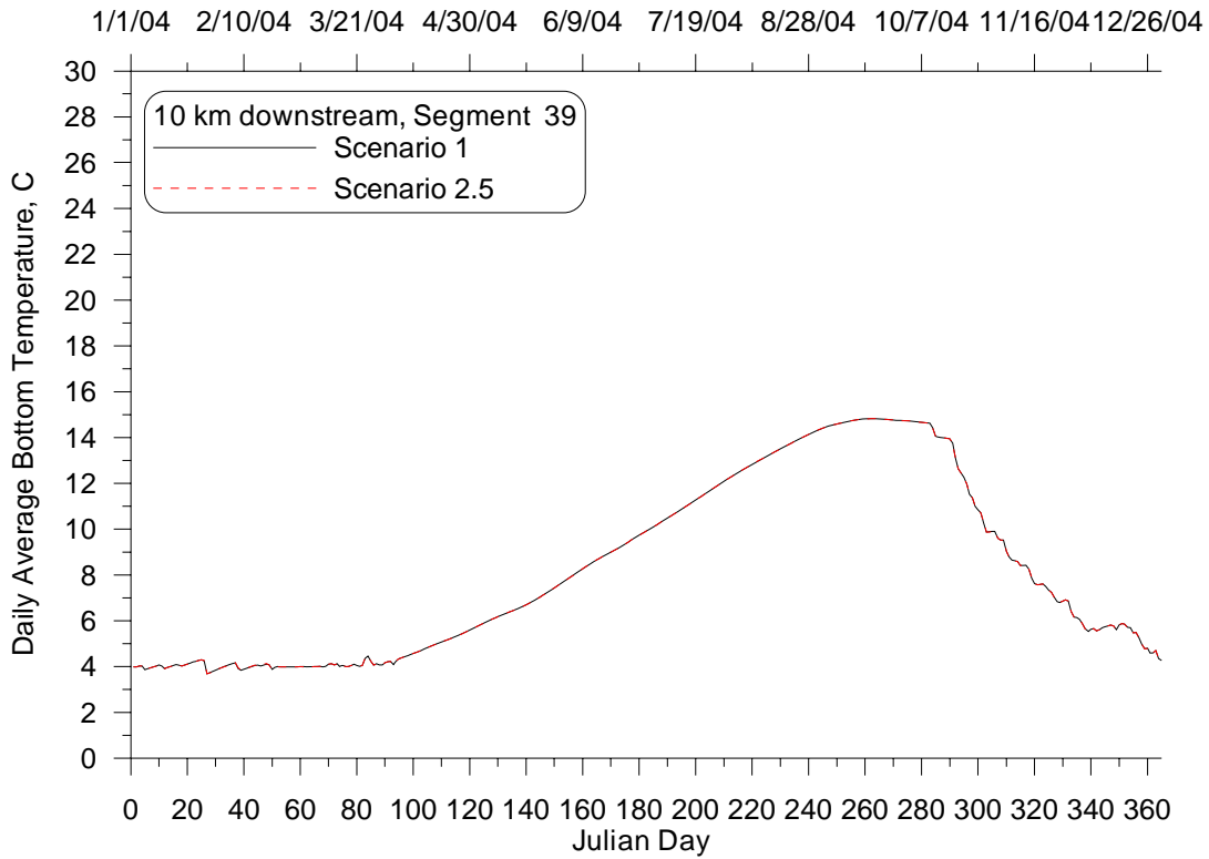
Figure 34: Daily average bottom temperature time series at 10 km downstream from Lake Pend Oreille for the Impounded with no NPS (2.5) and Existing Conditions (1) Scenarios, 2004.
