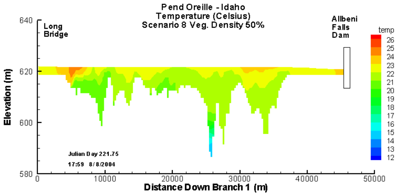
Figure 20: Longitudinal temperature profile for Model Scenario 8, Natural Conditions on August 8 th , 2004.
