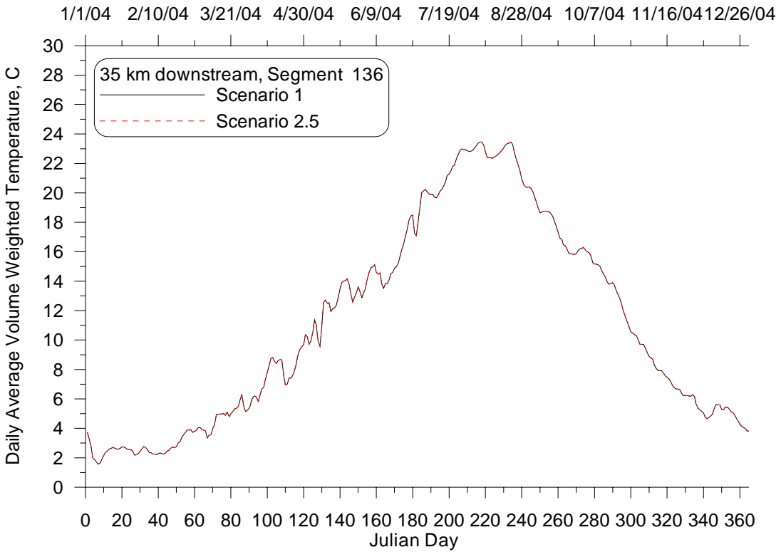
Figure 38: Daily average volume weighted temperature time series at 35 km downstream from Lake Pend Oreille for the Impounded with no NPS (2.5) and Existing Conditions (1) Scenarios, 2004.
