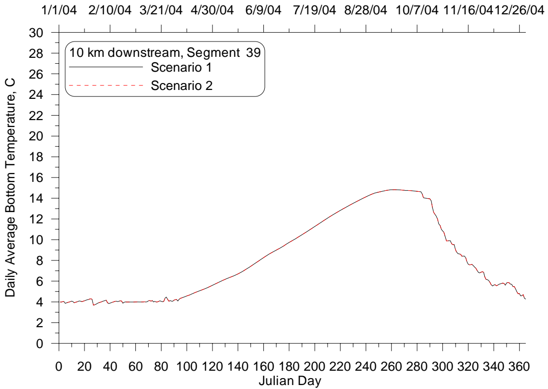
Figure 23: Daily average bottom temperature time series at 10 km downstream from Lake Pend Oreille for the Impounded with no NPDES (2) and Existing Conditions (1) Scenarios, 2004.
