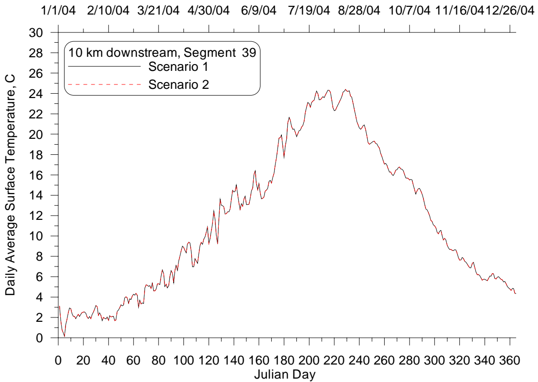
Figure 22: Daily average surface temperature time series at 10 km downstream from Lake Pend Oreille for the Impounded with no NPDES (2) and Existing Conditions (1) Scenarios, 2004.
