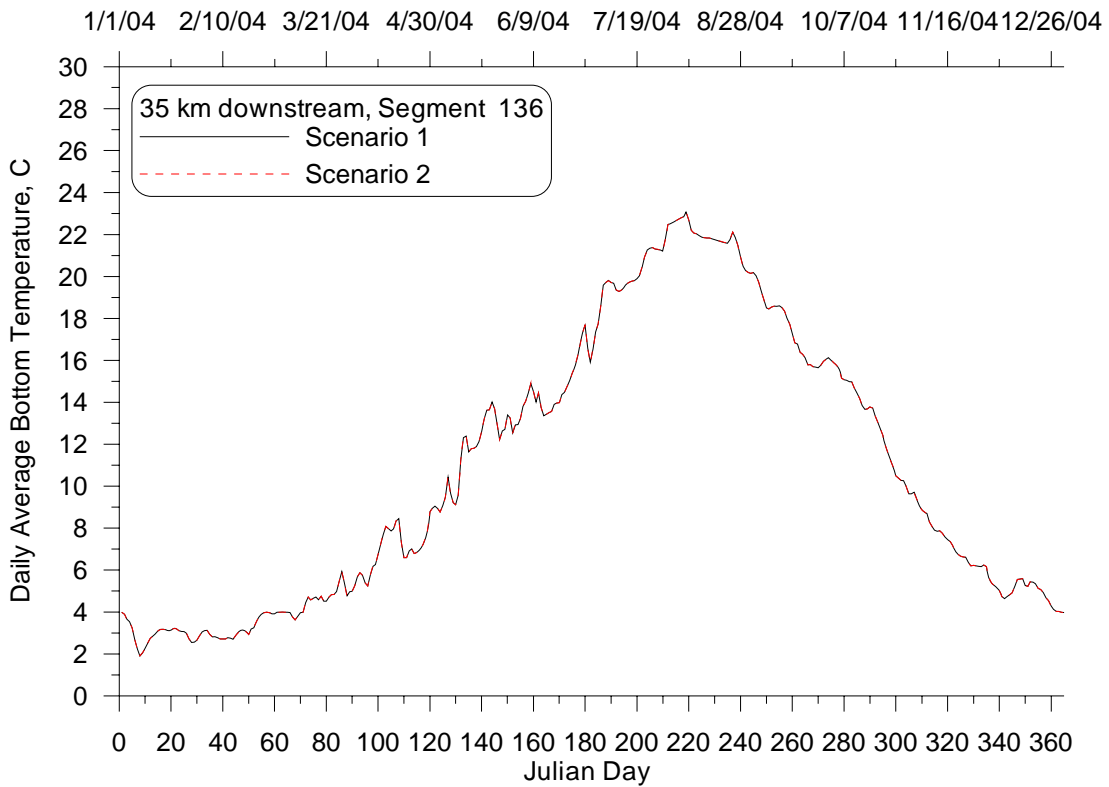
Figure 26: Daily average bottom temperature time series at 35 km downstream from Lake Pend Oreille for the Impounded with no NPDES (2) and Existing Conditions (1) Scenarios, 2004.
