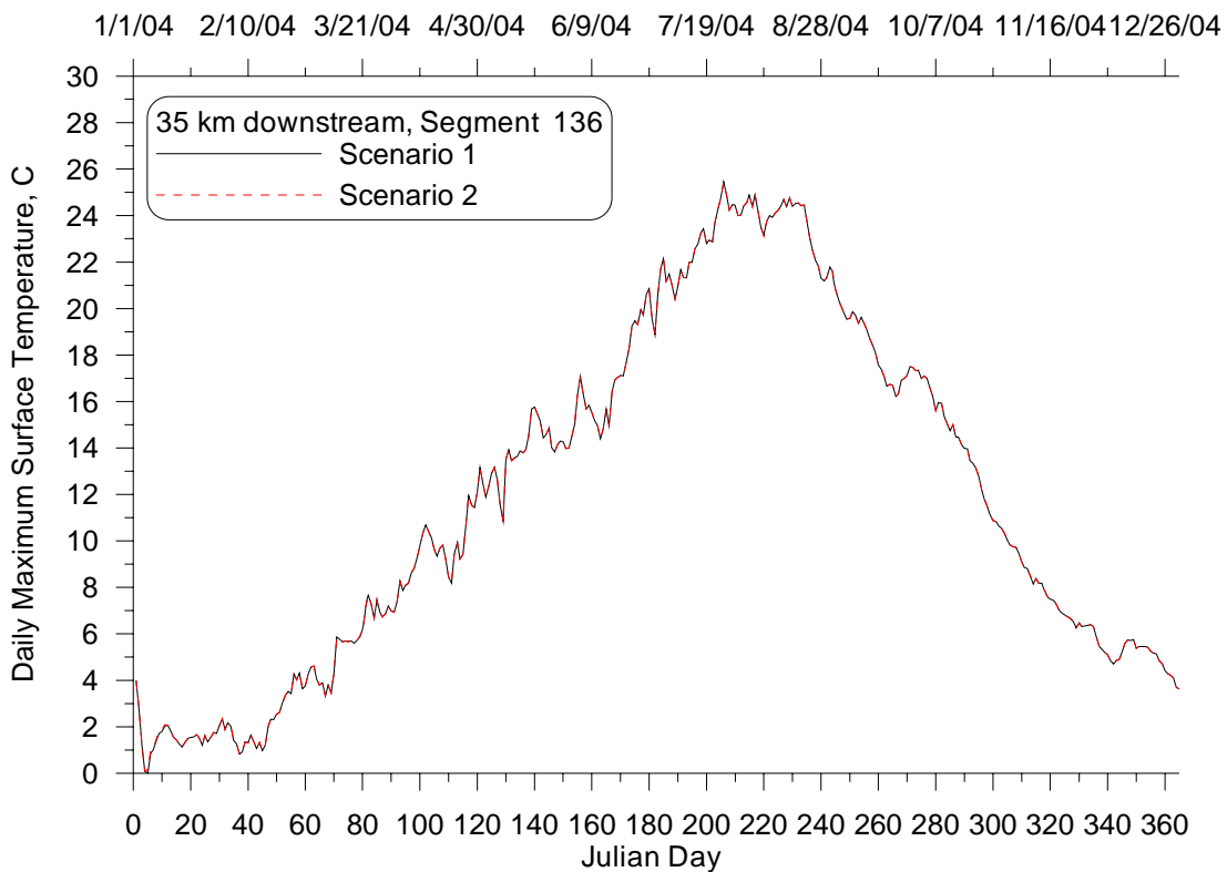
Figure 30: Daily maximum surface temperature time series at 35 km downstream from Lake Pend Oreille for the Impounded with no NPDES (2) and Existing Conditions (1) Scenarios, 2004.
