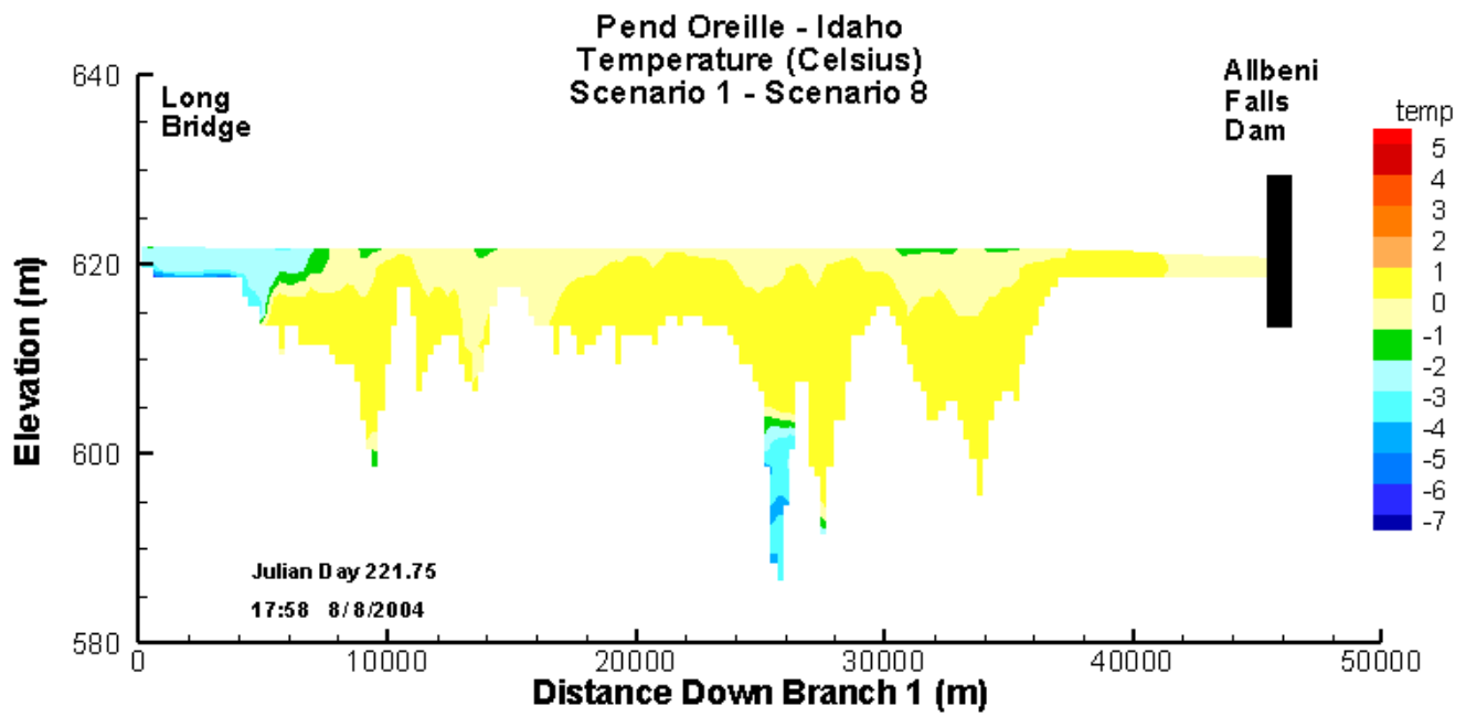
Figure 21: Longitudinal temperature profile difference, Existing Conditions (1) - Natural Conditions (8) Scenarios on August 8 th , 2004.
