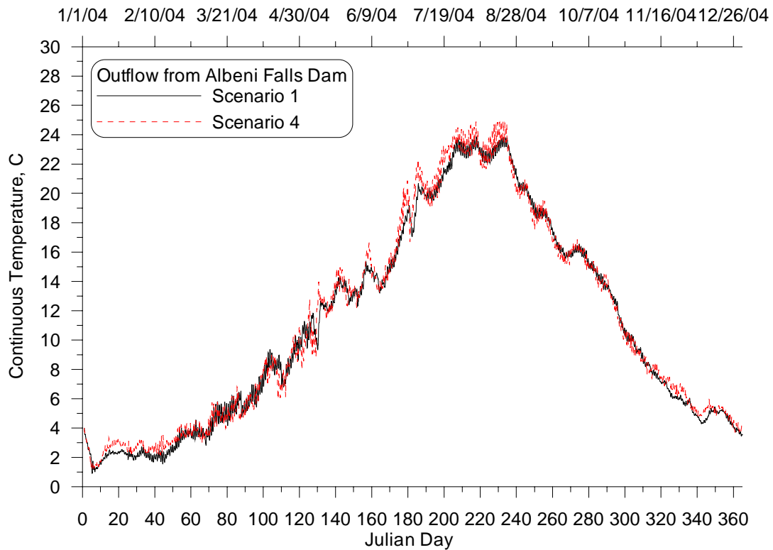
Figure 50: Continuous outflow temperature time series at Albeni Falls Dam for the Unimpounded (4) and Existing Conditions (1) Scenarios, 2004.
