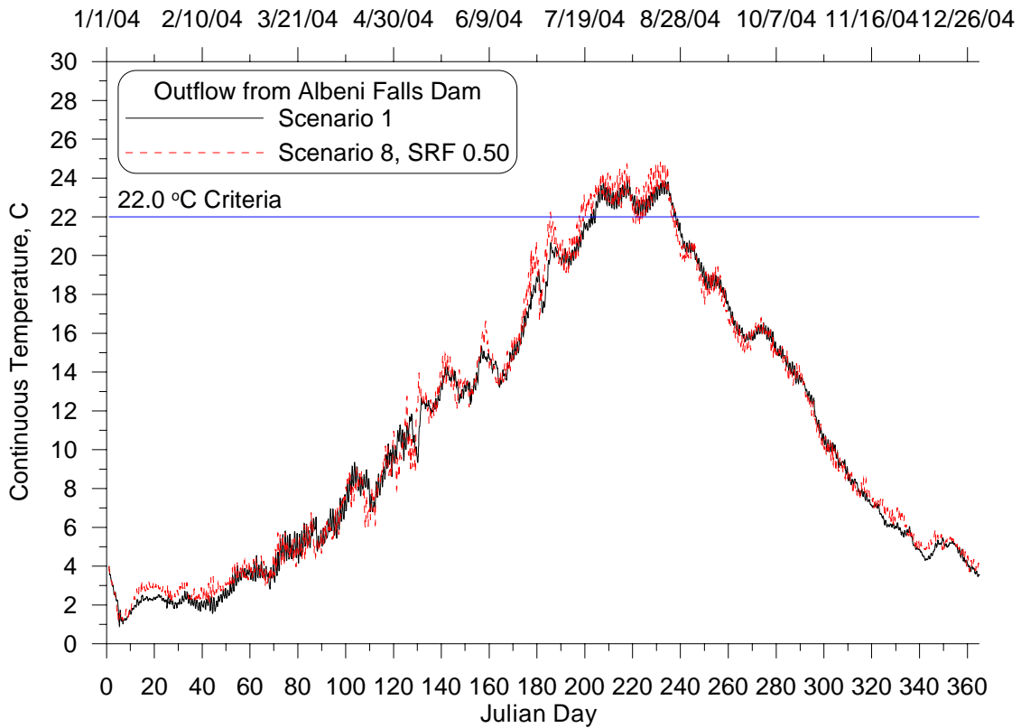
Figure 9: Continuous outflow temperature time series at Albeni Falls Dam for the Natural Conditions (8) and Existing Conditions (1) Scenarios, 2004.
