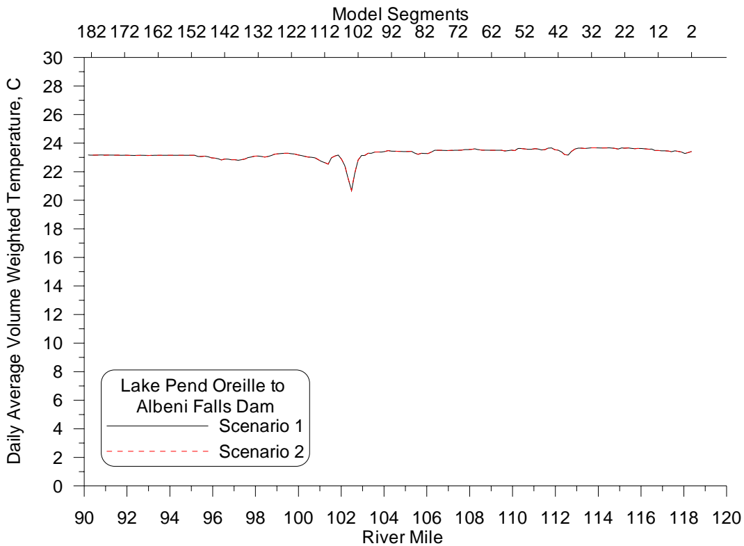
Figure 32: Daily average volume weighted temperature longitudinal profile on August 16 th , 2004 for the Impounded with no NPDES (2) and Existing Conditions (1) Scenarios.
