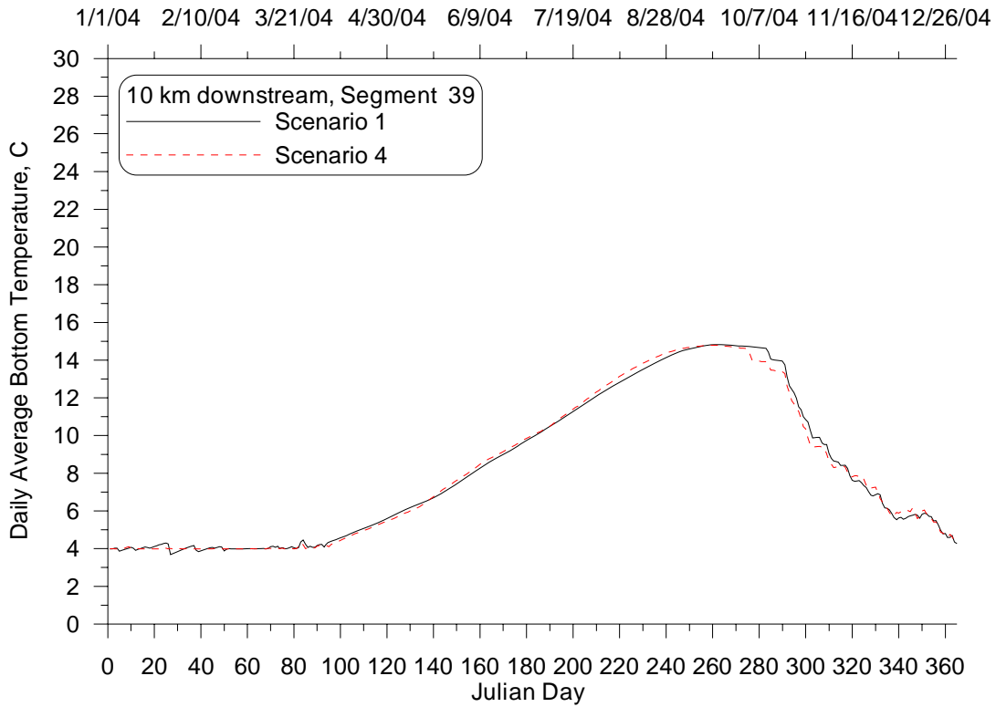
Figure 45: Daily average bottom temperature time series at 10 km downstream from Lake Pend Oreille for the Unimpounded (4) and Existing Conditions (1) Scenarios, 2004.
