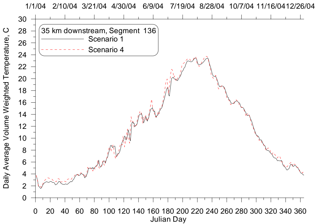
Figure 49: Daily average volume weighted temperature time series at 35 km downstream from Lake Pend Oreille for the Unimpounded (4) and Existing Conditions (1) Scenarios, 2004.
