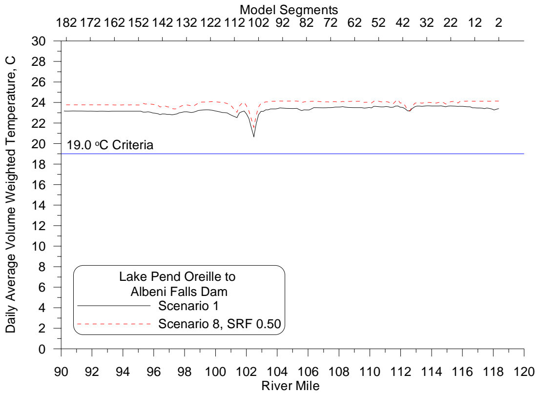
Figure 15: Daily average volume-weighted temperature longitudinal profile on August 16 th , 2004 for the Natural Conditions (8) and Existing Conditions (1) Scenarios.
