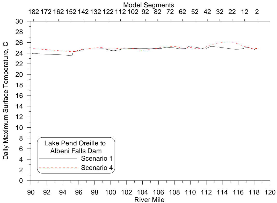
Figure 54: Daily maximum surface temperature longitudinal profile on August 16 th , 2004 for the Unimpounded (4) and Existing Conditions (1) Scenarios.
