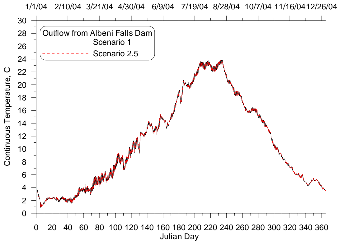
Figure 39: Continuous outflow temperature time series at Albeni Falls Dam for the Impounded with no NPS (2.5) and Existing Conditions (1) Scenarios, 2004.
