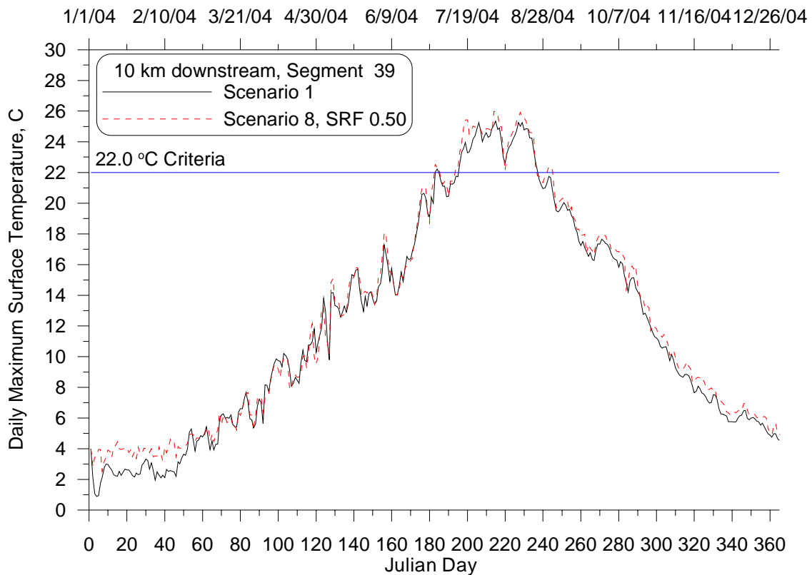
Figure 10: Daily maximum surface temperature time series at 10 km downstream from Lake Pend Oreille for the Natural Conditions (8) and Existing Conditions (1) Scenarios, 2004.
