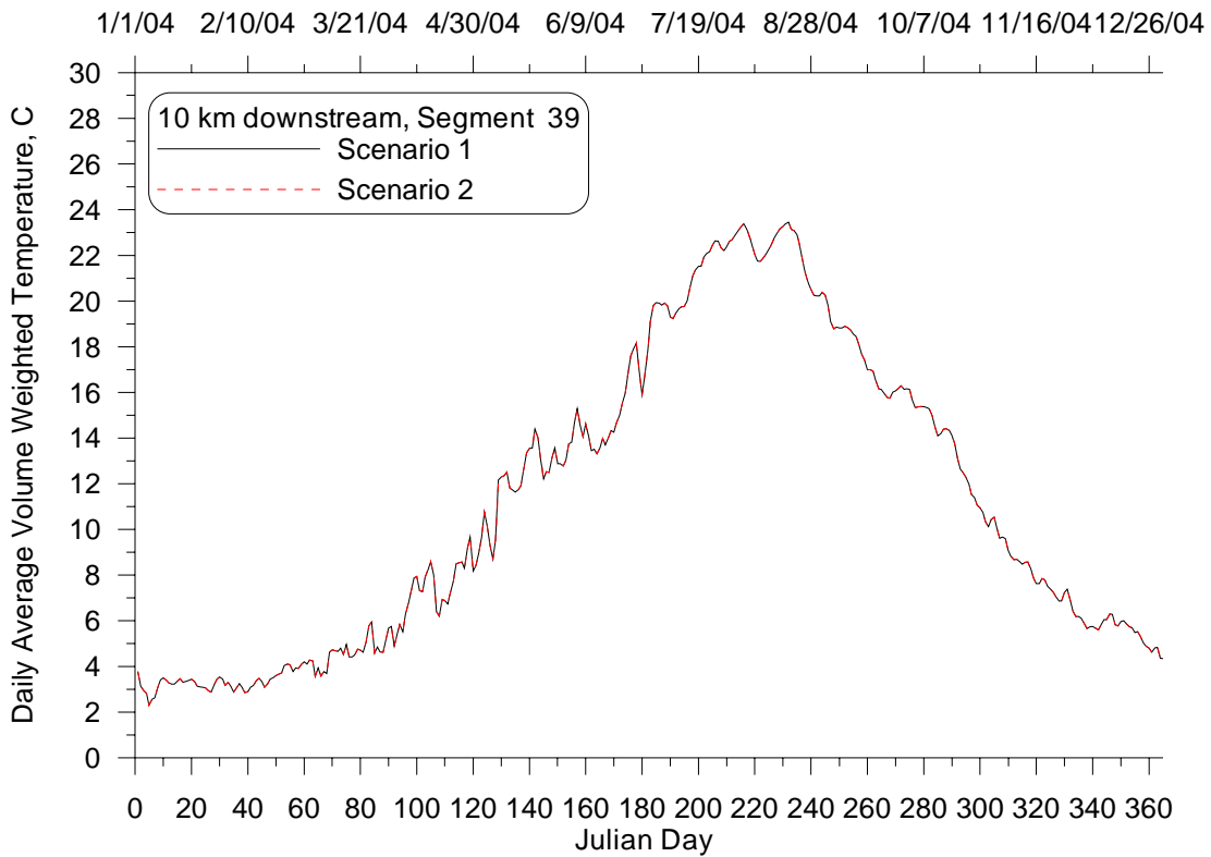
Figure 24: Daily average volume weighted temperature time series at 10 km downstream from Lake Pend Oreille for the Impounded with no NPDES (2) and Existing Conditions (1) Scenarios, 2004.
