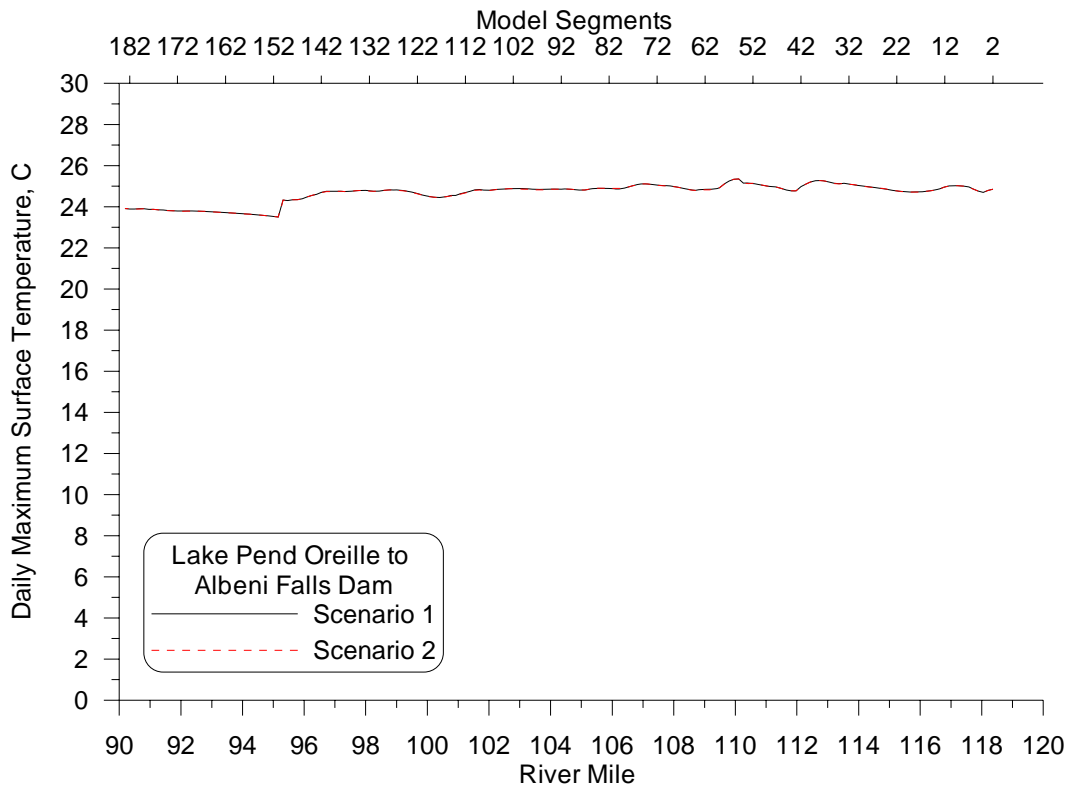
Figure 31: Daily maximum surface temperature longitudinal profile on August 16 th , 2004 for the Impounded with no NPDES (2) and Existing Conditions (1) Scenarios.
