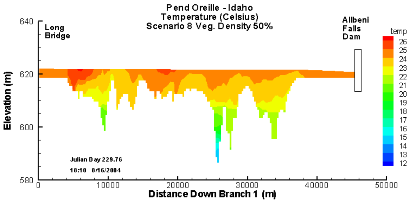
Figure 17: Longitudinal temperature profile for Model Scenario 8, Natural Conditions on August 16 th , 2004.
