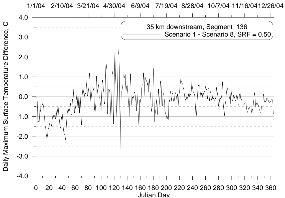
Figure 13: Daily maximum surface temperature difference time series at 35 km downstream from Lake Pend Oreille between the Natural Conditions (8) and Existing Conditions (1) Scenarios, 2004.
