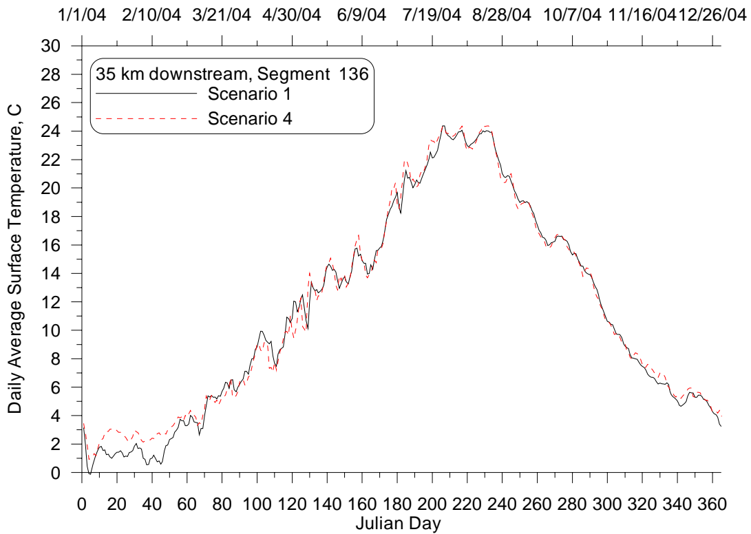
Figure 47: Daily average surface temperature time series at 35 km downstream from Lake Pend Oreille for the Unimpounded (4) and Existing Conditions (1) Scenarios, 2004.
