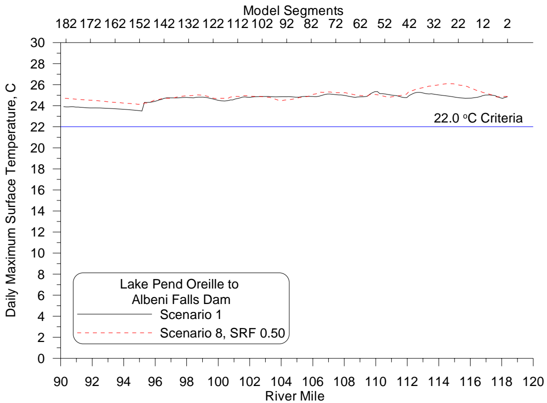
Figure 14: Daily maximum surface temperature longitudinal profile on August 16 th , 2004 for the Natural Conditions (8) and Existing Conditions (1) Scenarios.
