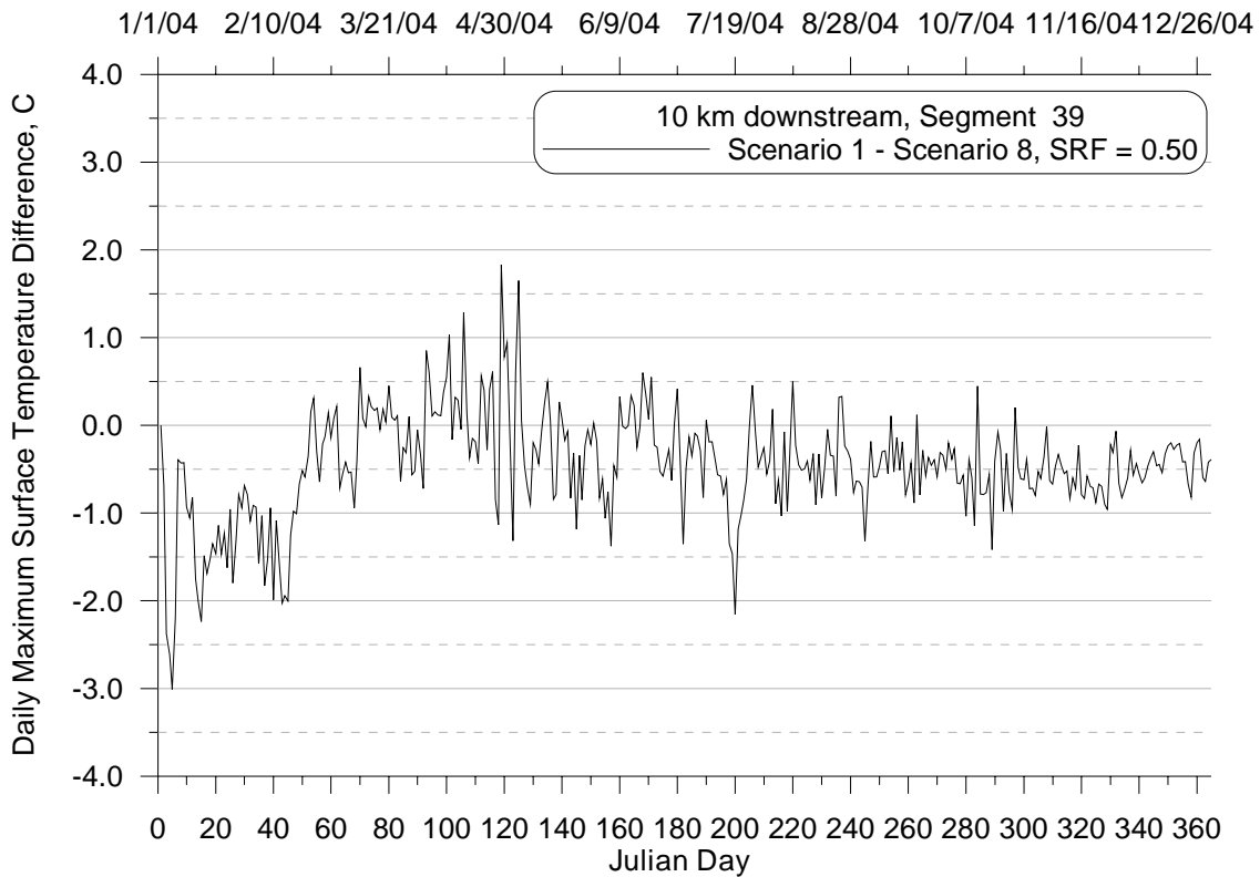
Figure 11: Daily maximum surface temperature difference time series at 10 km downstream from Lake Pend Oreille between the Natural Conditions (8) and Existing Conditions (1) Scenarios, 2004.
