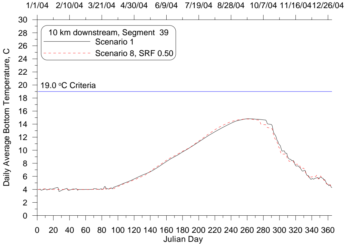
Figure 4: Daily average bottom temperature time series at 10 km downstream from Lake Pend Oreille for the Natural Conditions (8) and Existing Conditions (1) Scenarios, 2004.
