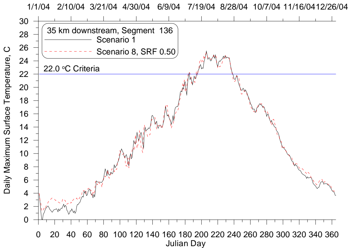
Figure 12: Daily maximum surface temperature time series at 35 km downstream from Lake Pend Oreille for the Natural Conditions (8) and Existing Conditions (1) Scenarios, 2004.
