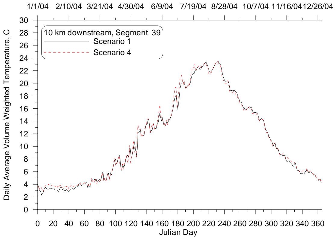
Figure 46: Daily average volume weighted temperature time series at 10 km downstream from Lake Pend Oreille for the Unimpounded (4) and Existing Conditions (1) Scenarios, 2004.
