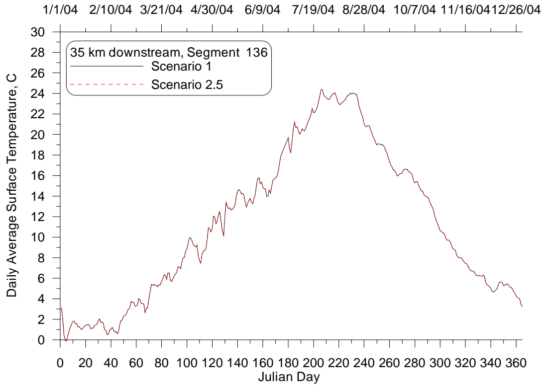
Figure 36: Daily average surface temperature time series at 35 km downstream from Lake Pend Oreille for the Impounded with no NPS (2.5) and Existing Conditions (1) Scenarios, 2004.
