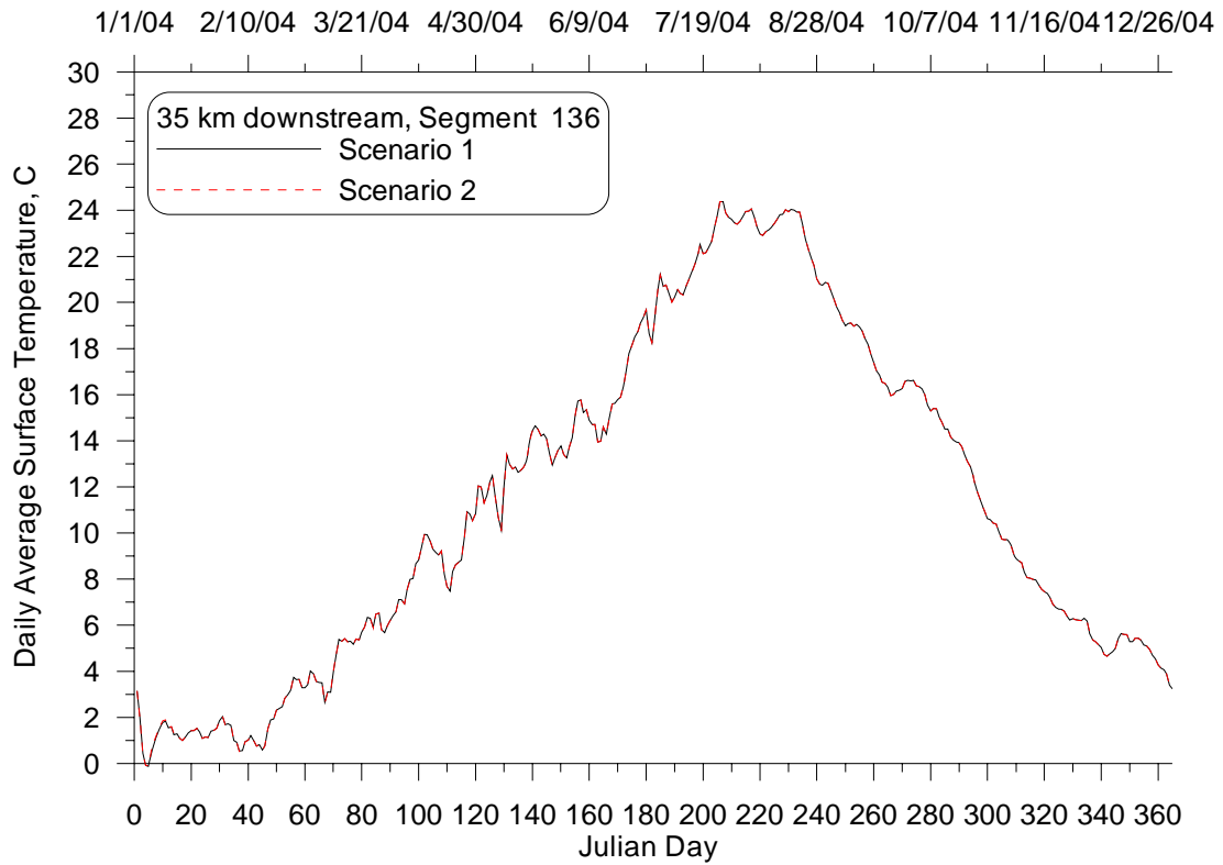
Figure 25: Daily average surface temperature time series at 35 km downstream from Lake Pend Oreille for the Impounded with no NPDES (2) and Existing Conditions (1) Scenarios, 2004.
