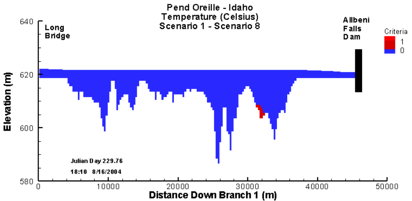
Figure 58: Longitudinal temperature profile difference, Existing Conditions (1) - Natural Conditions (8) Scenarios on August 16 th , 2004 red indicates temperature difference was above 0.3 °C and river temperature was above 22 °C.
