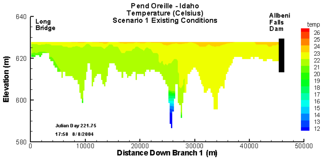
Figure 19: Longitudinal temperature profile for Model Scenario 1, Existing Conditions on August 8th, 2004.
