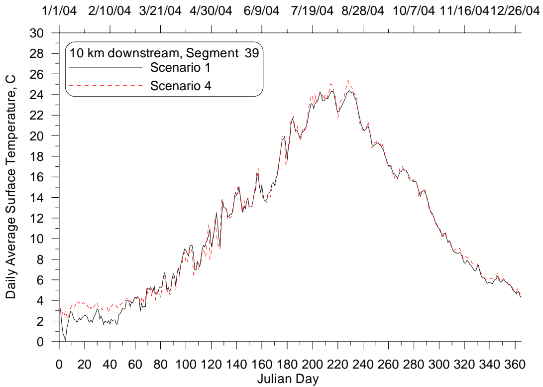
Figure 44: Daily average surface temperature time series at 10 km downstream from Lake Pend Oreille for the Unimpounded (4) and Existing Conditions (1) Scenarios, 2004.
