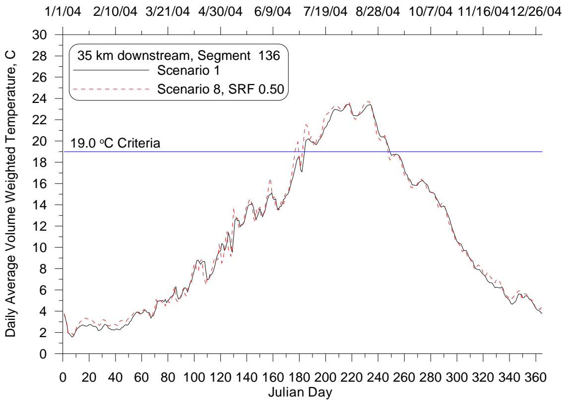
Figure 8: Daily average volume weighted temperature time series at 35 km downstream from Lake Pend Oreille for the Natural Conditions (8) and Existing Conditions (1) Scenarios, 2004.
