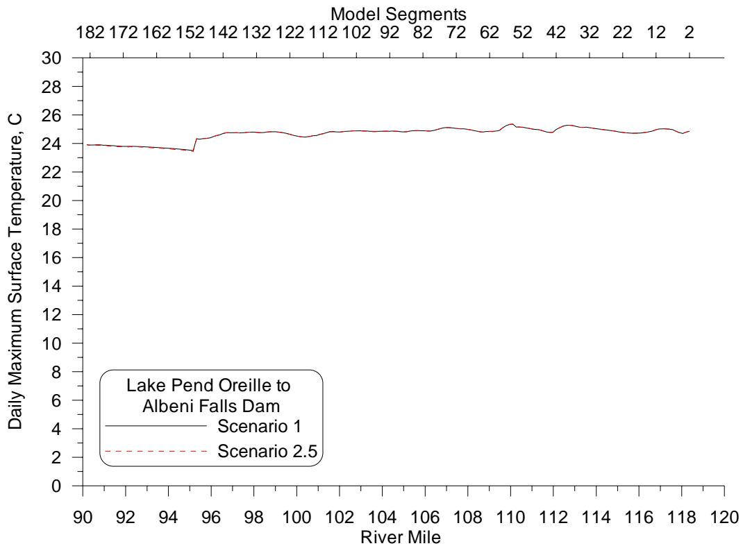
Figure 42: Daily maximum surface temperature longitudinal profile on August 16 th , 2004 for the Impounded with no NPS (2.5) and Existing Conditions (1) Scenarios.
