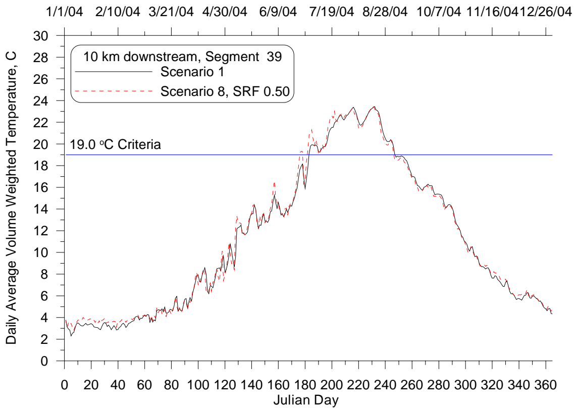
Figure 5: Daily average volume weighted temperature time series at 10 km downstream from Lake Pend Oreille for the Natural Conditions (8) and Existing Conditions (1) Scenarios, 2004.
