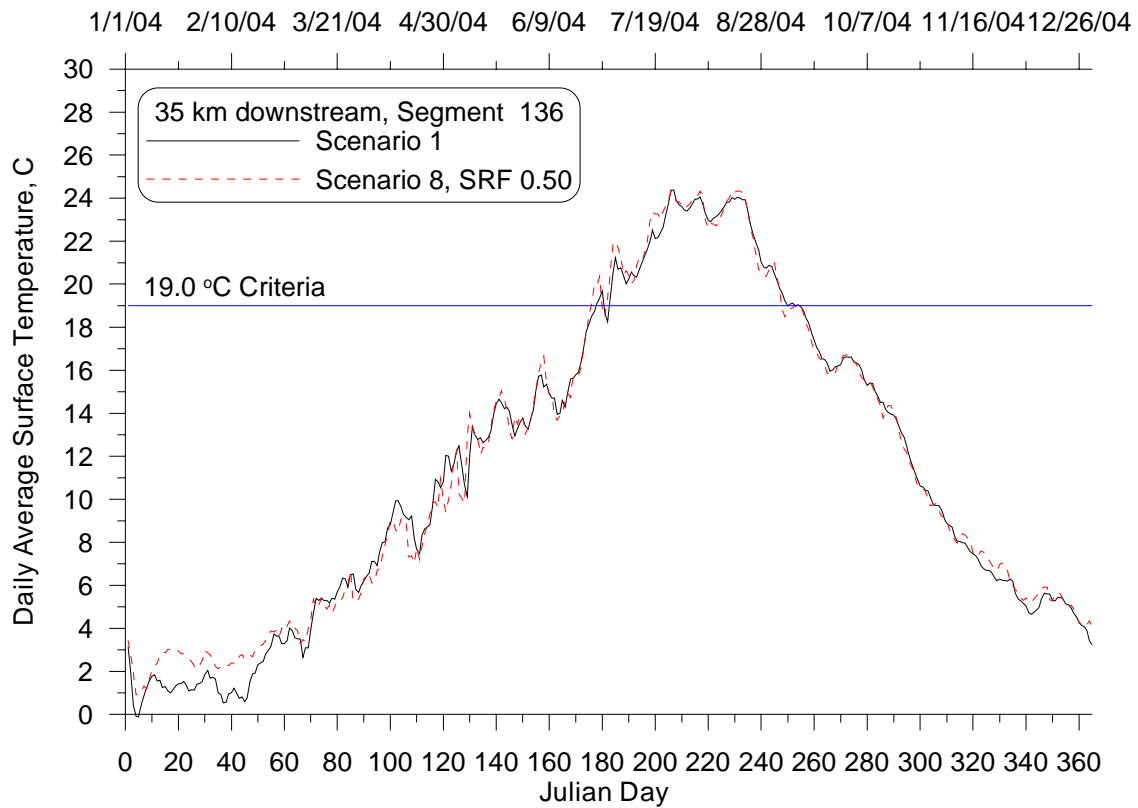
Figure 6: Daily average surface temperature time series at 35 km downstream from Lake Pend Oreille for the Natural Conditions (8) and Existing Conditions (1) Scenarios 2004.
