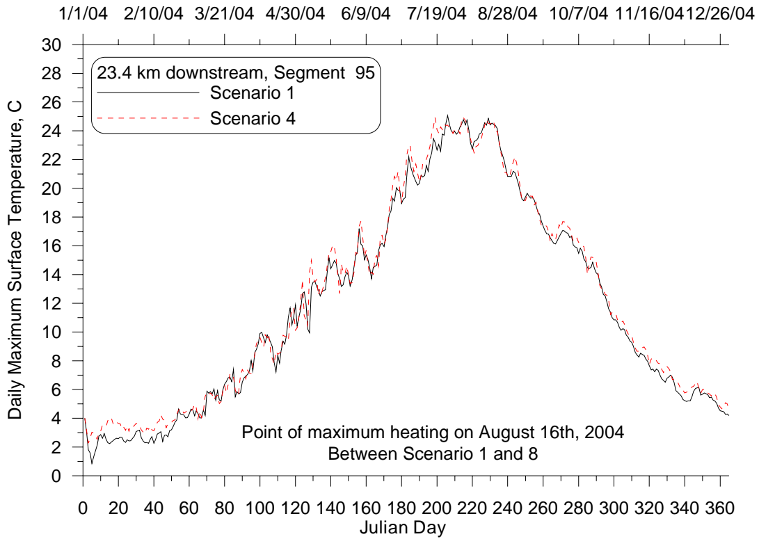
Figure 53: Daily maximum surface temperature time series at 23.4 km downstream from Long Bridge for the Unimpounded (4) and Existing Conditions (1) Scenarios, 2004. Based on the point of maximum heating on August 16 th , 2004 between the Existing Conditions (1) and Natural Conditions (8) Scenarios.
