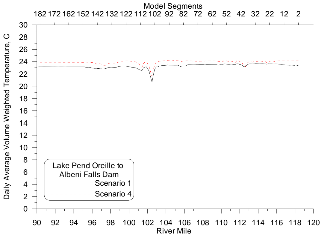
Figure 55: Daily average volume weighted temperature longitudinal profile on August 16 th , 2004 for the Unimpounded (4) and Existing Conditions (1) Scenarios.
