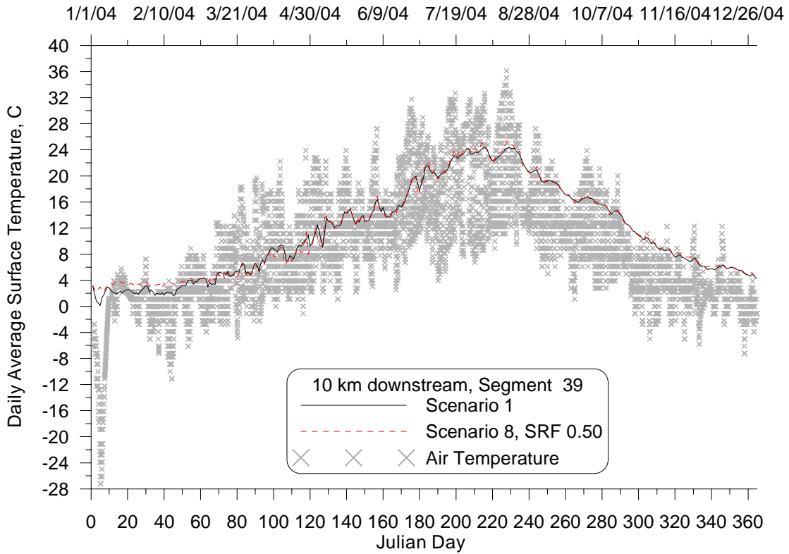
Figure 3: Daily average surface temperature time series at 10 km downstream from Lake Pend Oreille for the Natural Conditions (8) and Existing Conditions (1) Scenarios and Air Temperature, 2004.
