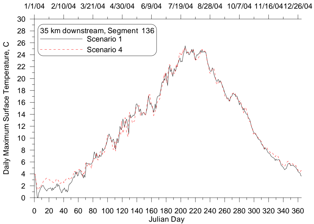
Figure 52: Daily maximum surface temperature time series at 35 km downstream from Lake Pend Oreille for the Unimpounded (4) and Existing Conditions (1) Scenarios, 2004.
