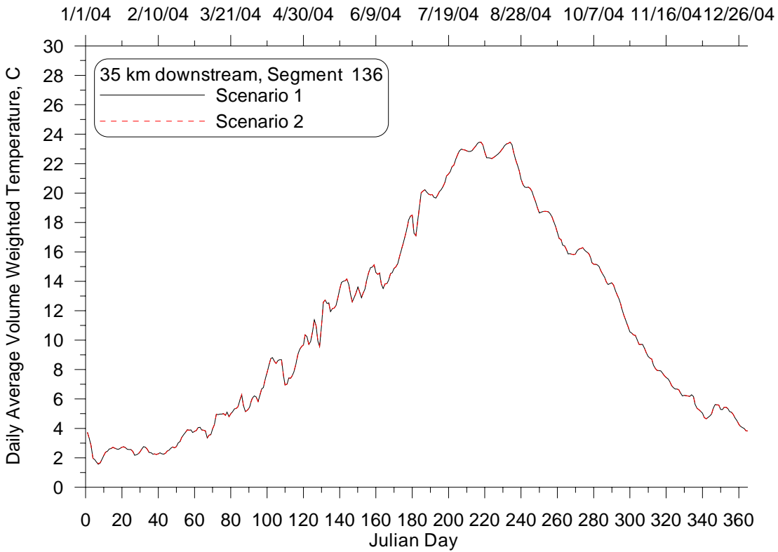
Figure 27: Daily average volume weighted temperature time series at 35 km downstream from Lake Pend Oreille for the Impounded with no NPDES (2) and Existing Conditions (1) Scenarios, 2004.
