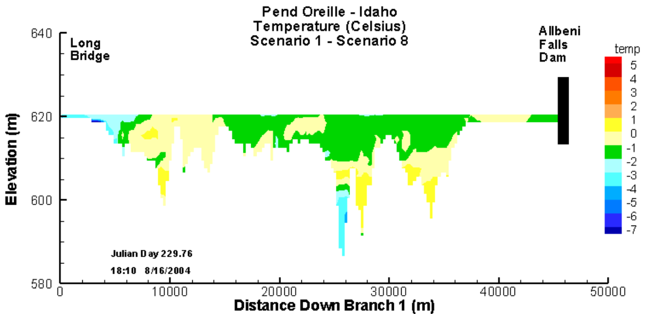
Figure 18: Longitudinal temperature profile difference, Existing Conditions (1) - Natural Conditions (8) Scenarios on August 16 th , 2004.
