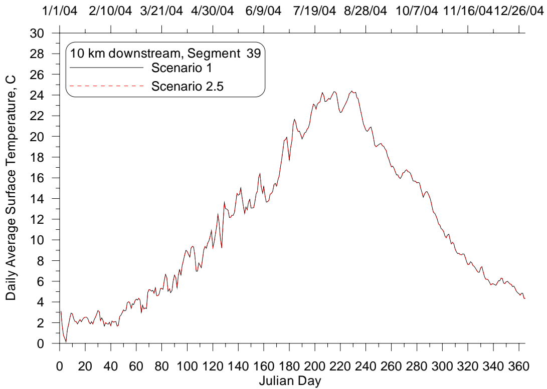
Figure 33: Daily average surface temperature time series at 10 km downstream from Lake Pend Oreille for the Impounded with no NPS (2.5) and Existing Conditions (1) Scenarios, 2004.
