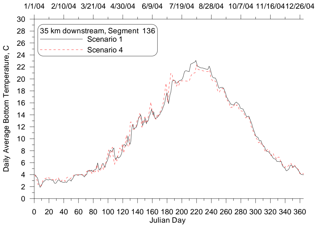
Figure 48: Daily average bottom temperature time series at 35 km downstream from Lake Pend Oreille for the Unimpounded (4) and Existing Conditions (1) Scenarios, 2004.
