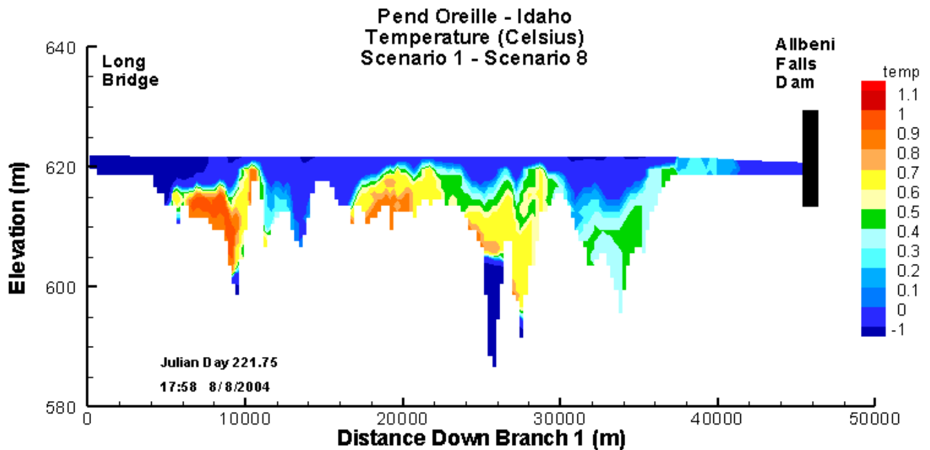
Figure 59: Longitudinal temperature profile difference, Existing Conditions (1) - Natural Conditions (8) Scenarios on August 8 th , 2004 with a refined temperature difference scale.
