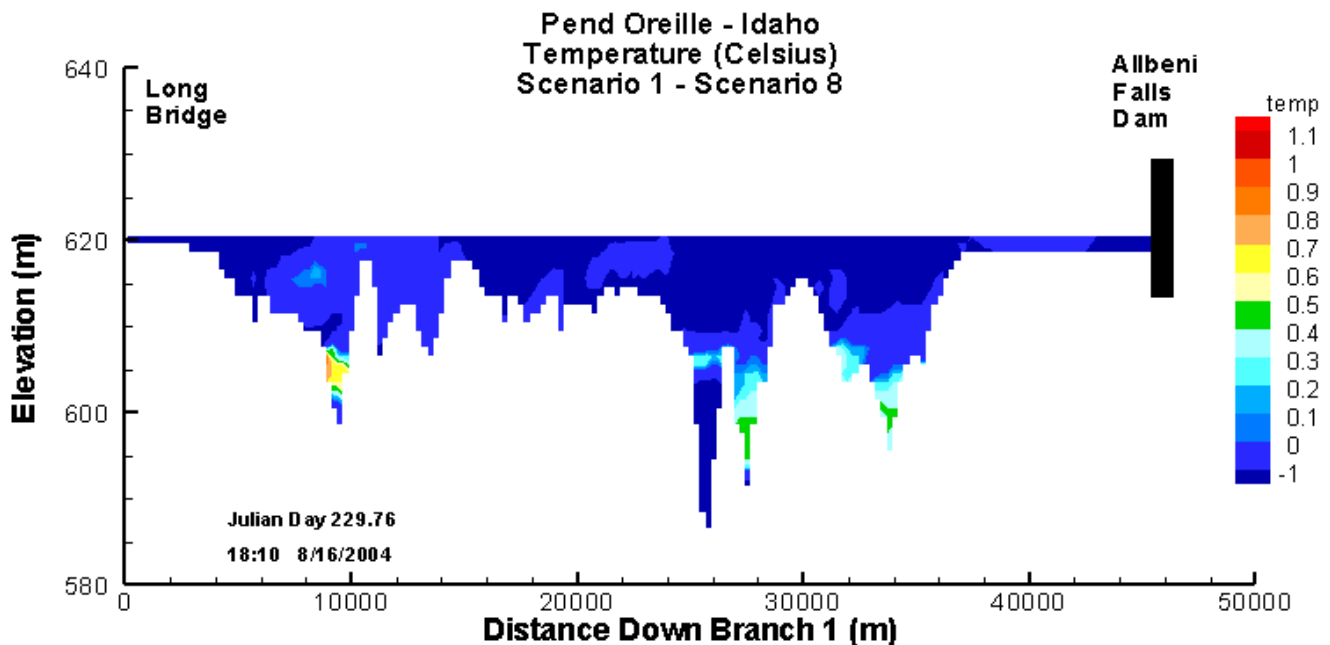
Figure 57: Longitudinal temperature profile difference, Existing Conditions (1) - Natural Conditions (8) Scenarios on August 16 th , 2004 with a refined temperature difference scale
