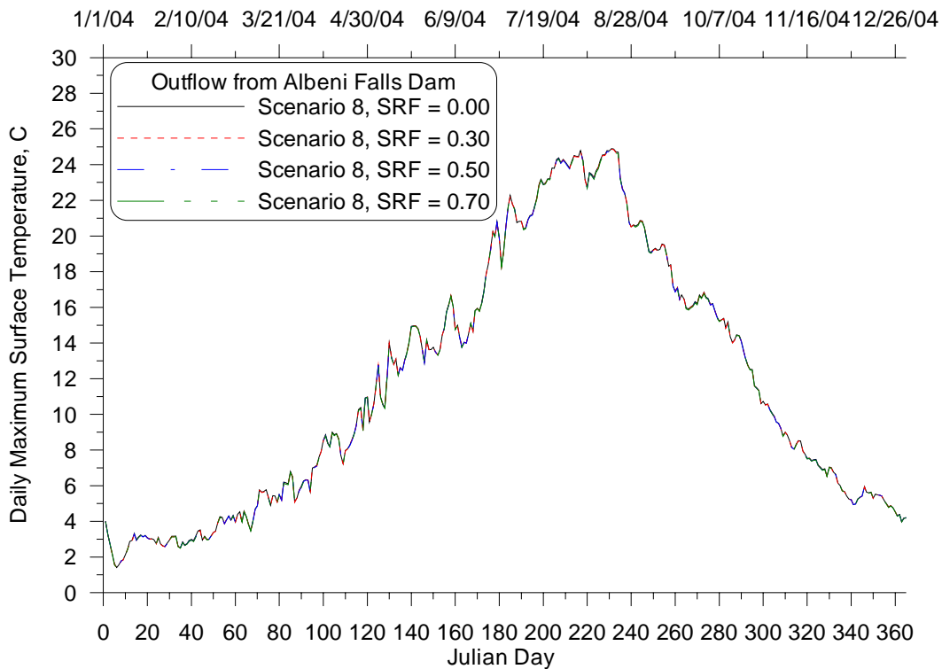
Figure 56: Daily maximum surface temperature time series at the Albeni Falls Dam location for Natural Conditions (8) Scenarios with various vegetation densities 2004.
