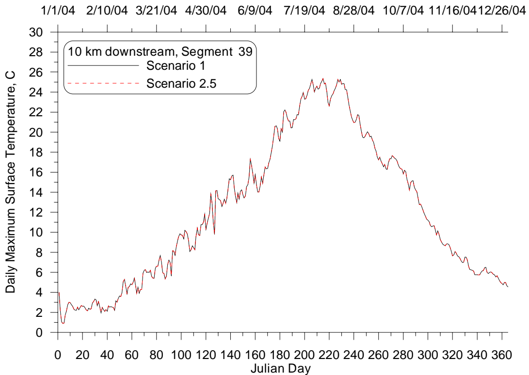
Figure 40: Daily maximum surface temperature time series at 10 km downstream from Lake Pend Oreille for the Impounded with no NPS (2.5) and Existing Conditions (1) Scenarios, 2004.
