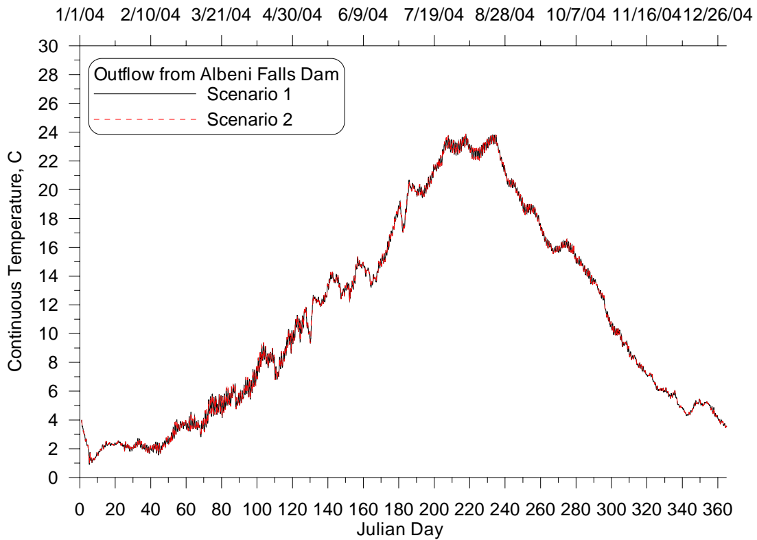
Figure 28: Continuous outflow temperature time series at Albeni Falls Dam for the Impounded with no NPDES (2) and Existing Conditions (1) Scenarios, 2004.
