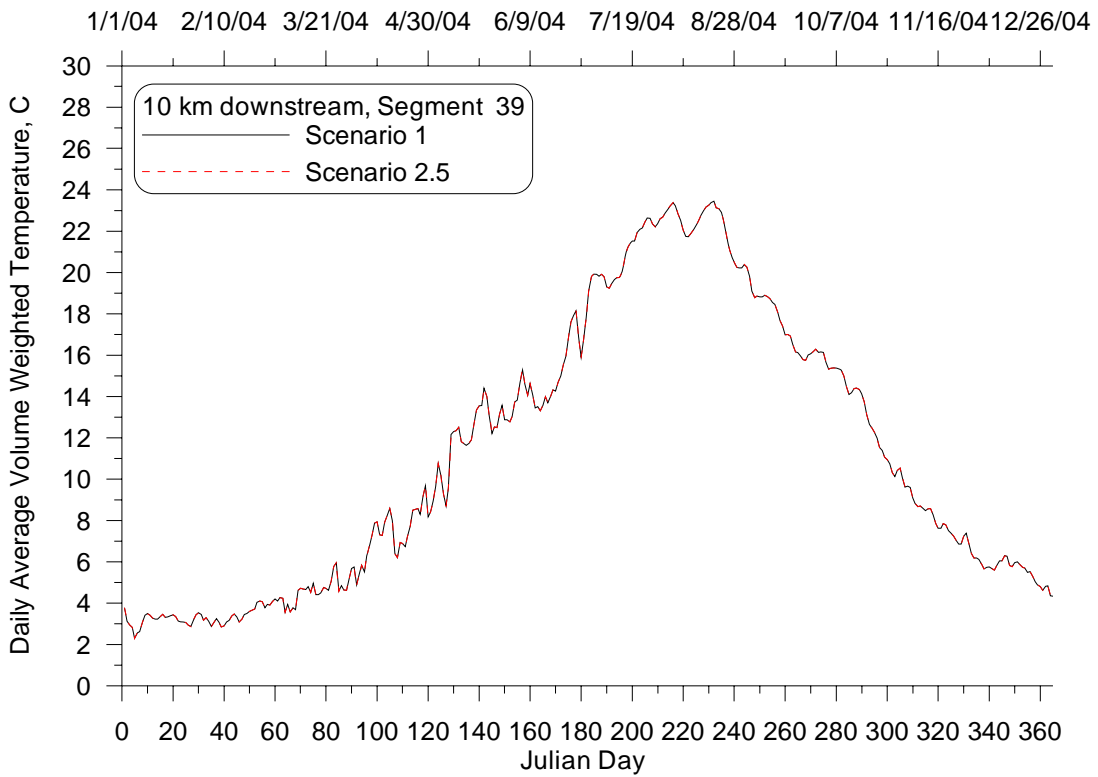
Figure 35: Daily average volume weighted temperature time series at 10 km downstream from Lake Pend Oreille for the Impounded with no NPS (2.5) and Existing Conditions (1) Scenarios, 2004.
